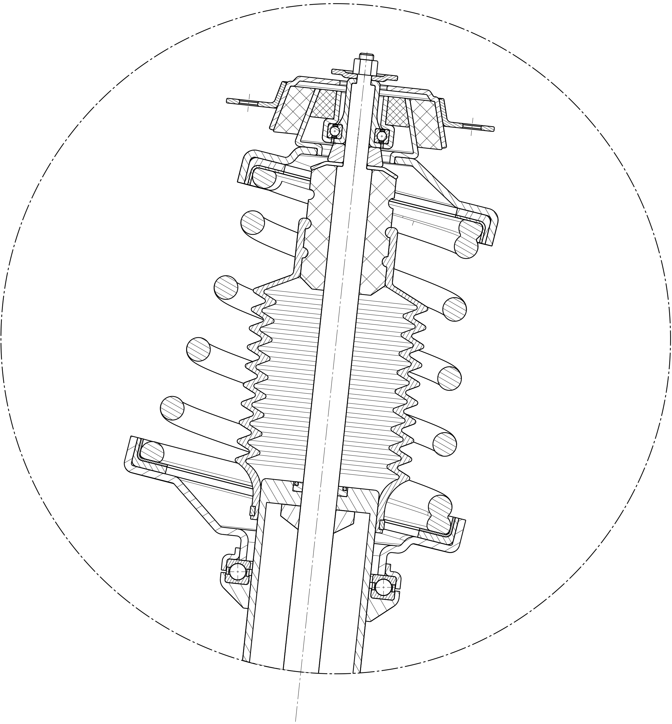
DETAIL B Scale (1:1)
